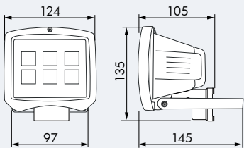
LED-6
