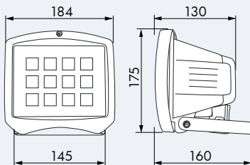
LED-12
