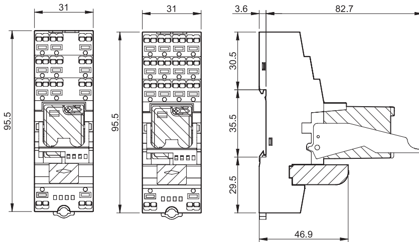
58.P3 Borne push-in
