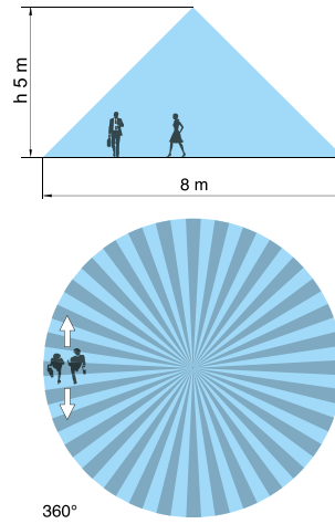
18.31.8.230.0000/18.21.8.230.0000 - Ceiling mounting
