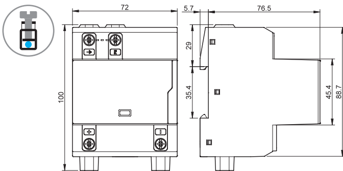
Type 7P.13.9.000.x006 Screw terminal
