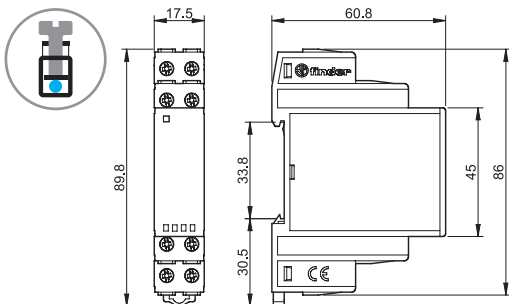
Type 7P.37.8.275.1003 Screw terminal
