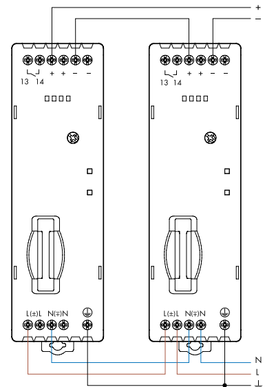
Series connection
