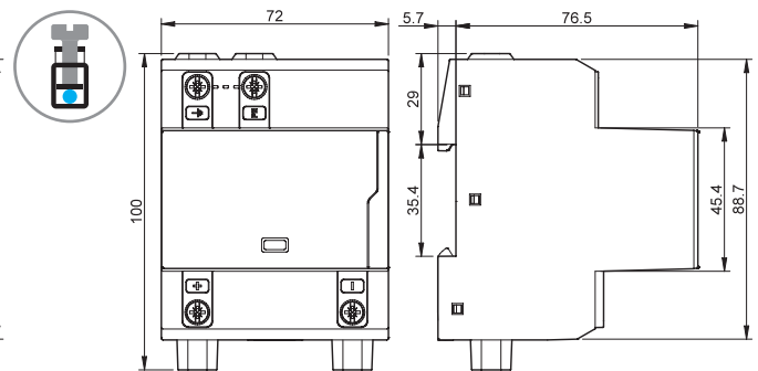
Type 7P.13.9.500.x006 Screw terminal
