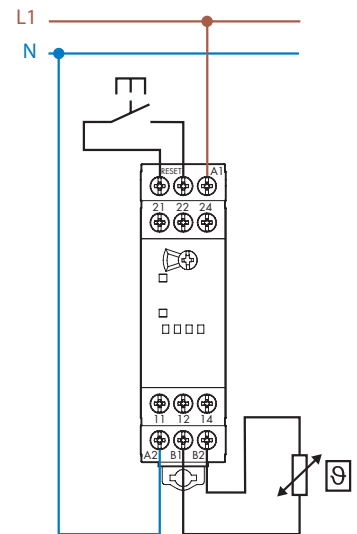
70.51 with TA connection
