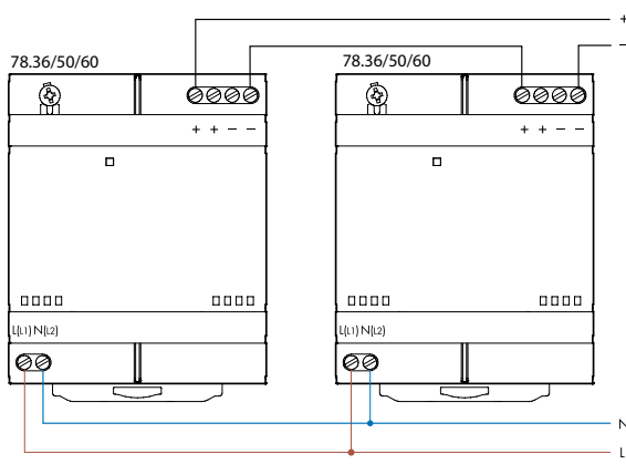
Series connection
