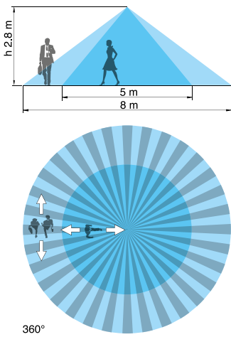
18.31...0031 - High ceilings installations
