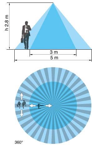
18.31...0031 - Internal ceiling installation, surface mounting
