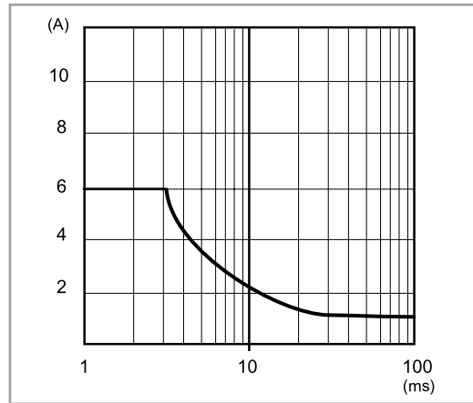
P78-3 Output peak current v time (78.36) - 24 V
