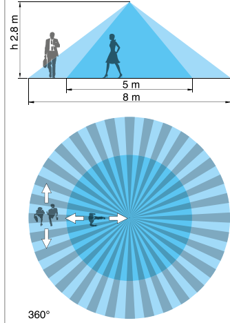
18.01, 18.11 - Ceiling mounting
