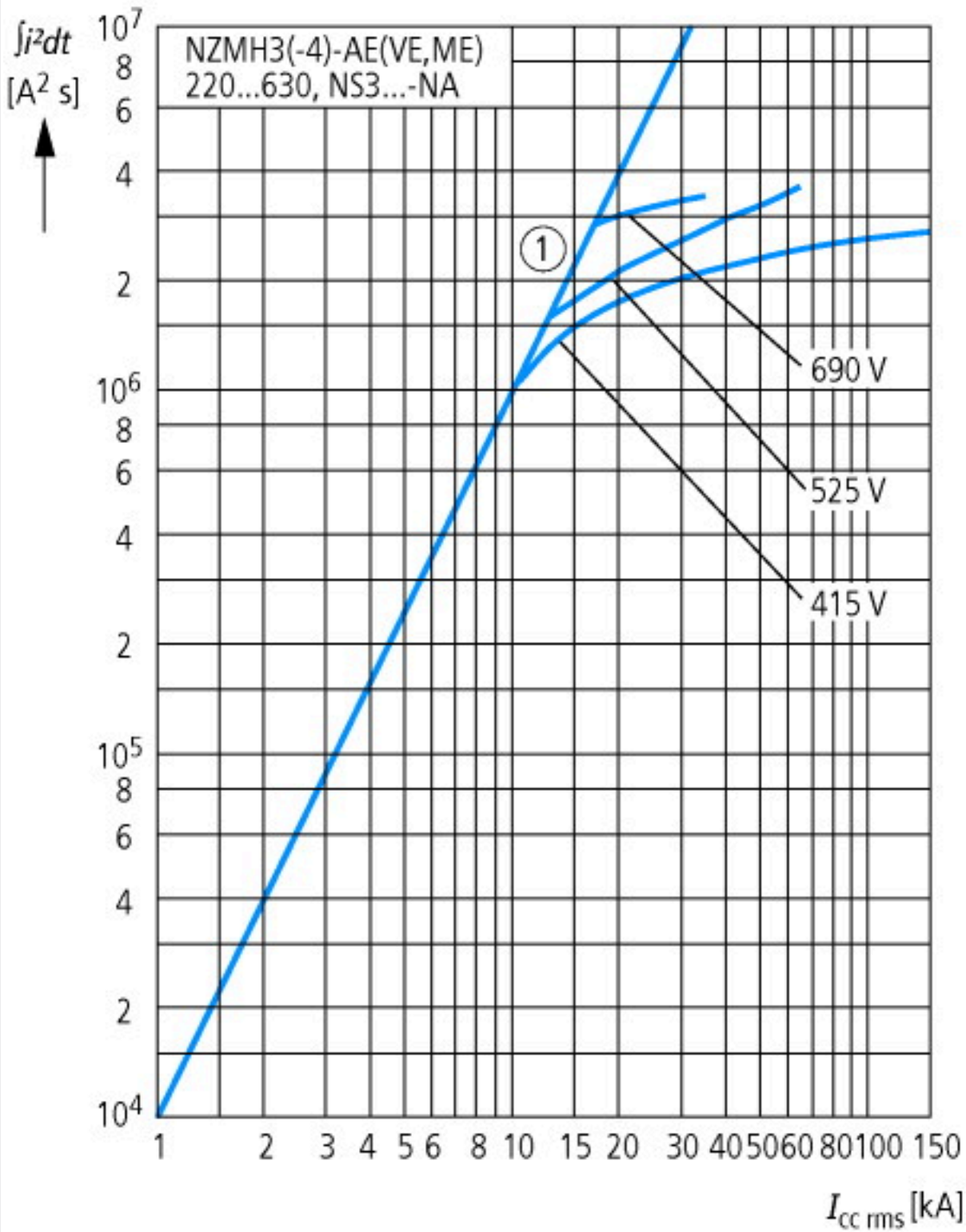
Let-through energy
