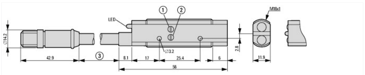
Sensor with installed adapter
