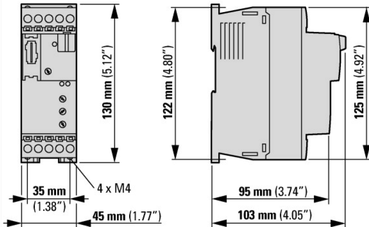
SmartWire-DT soft starter
