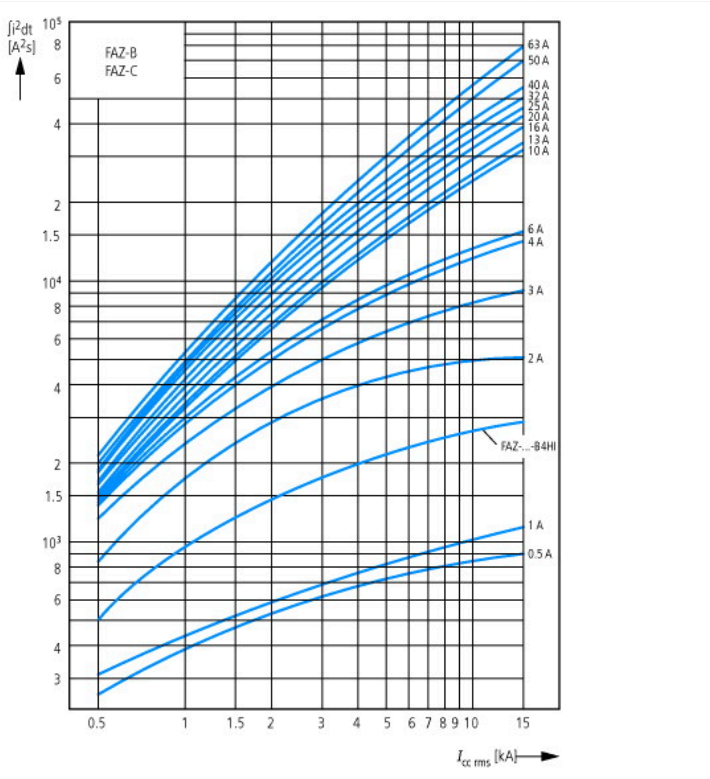
Let-through energy I^2t According to IEC/EN 60898
