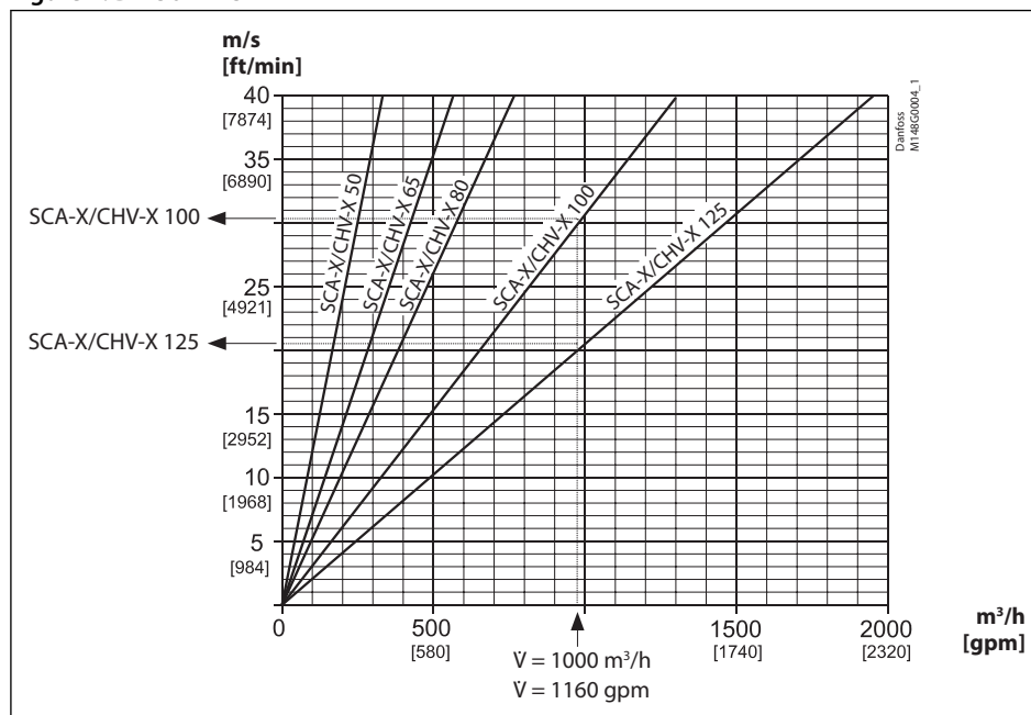
Figure 7: DN 50 - 125
