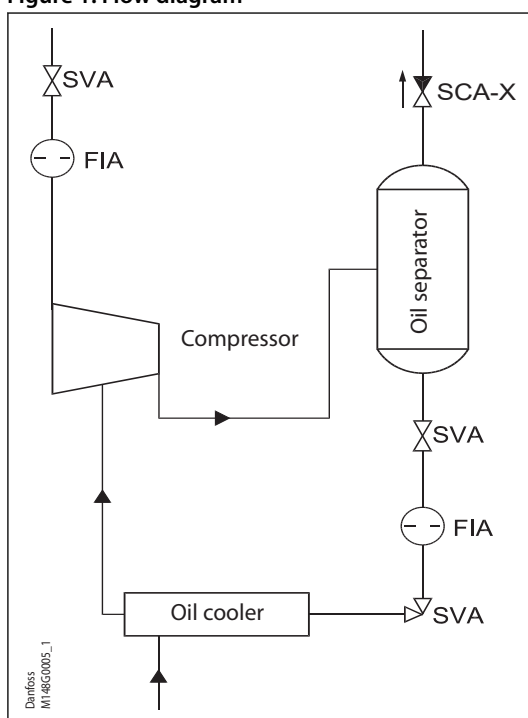
Figure 1: Flow diagram
