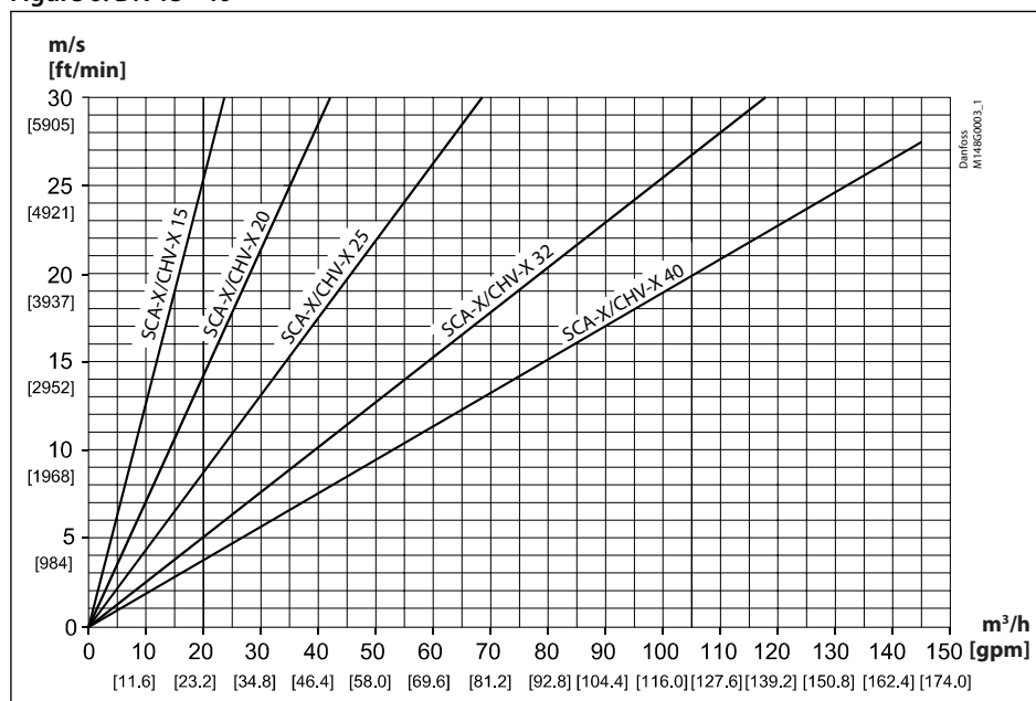
Figure 6: DN 15 - 40
