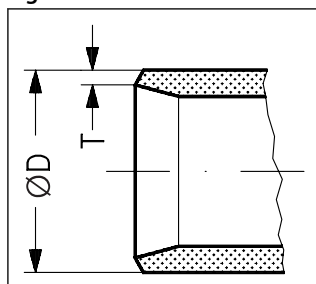
Figure 3: F connection
