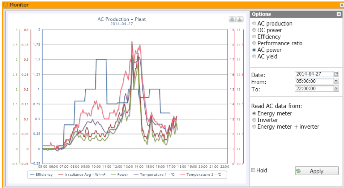
Figure 12: Monitor Window; AC Power Chart.
