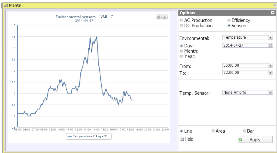
Figure 38: Plant Window; Sensor Chart "Temperature" - Options.
