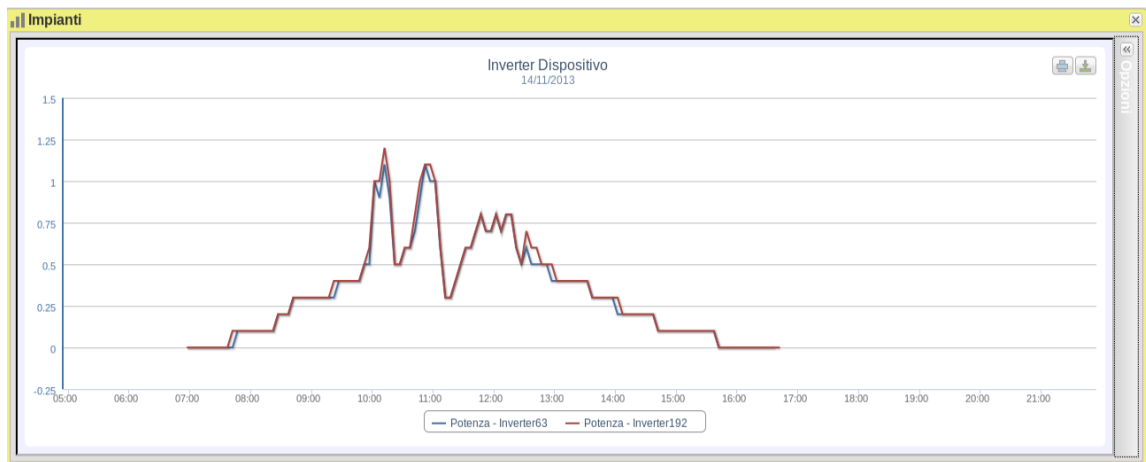
Figure 17: Plant Window; Inverter Chart – Option selection for Single Inverter.
