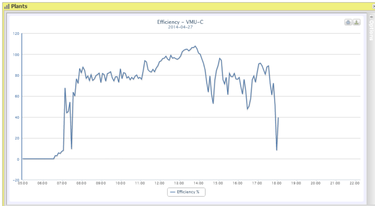
Figure 29: Plant Window; Efficiency Chart "All strings".
