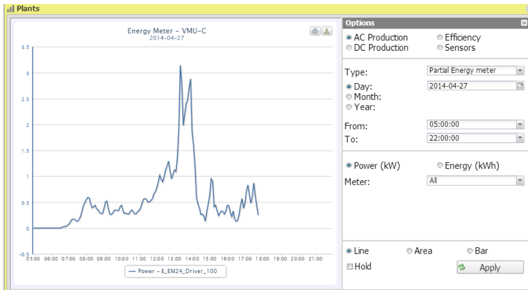
Figure 20: Plant Window; Energy Meter Chart– Option Selection for Partial Energy Meter.
