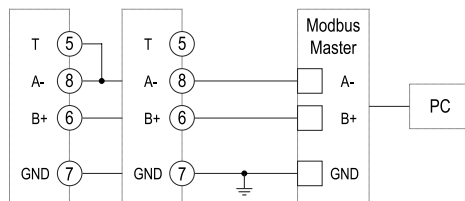
RS485 Modbus
