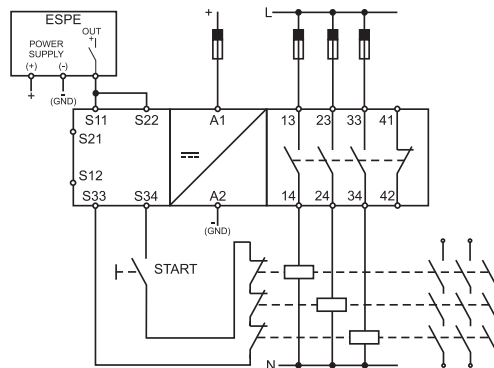
NLG13D - One 1-wire relay output - Safety cat. 2
