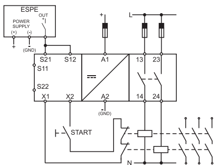
NLG02D - One 1-wire relay output - Safety cat. 2
