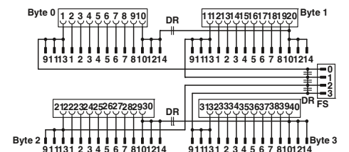
Connection scheme FLKM 50/4-FLK14/PA-S300
