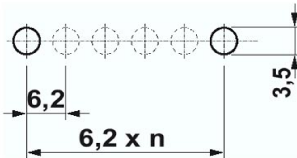
Drilling diagram
