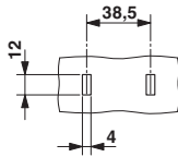
Dimensional drawing
