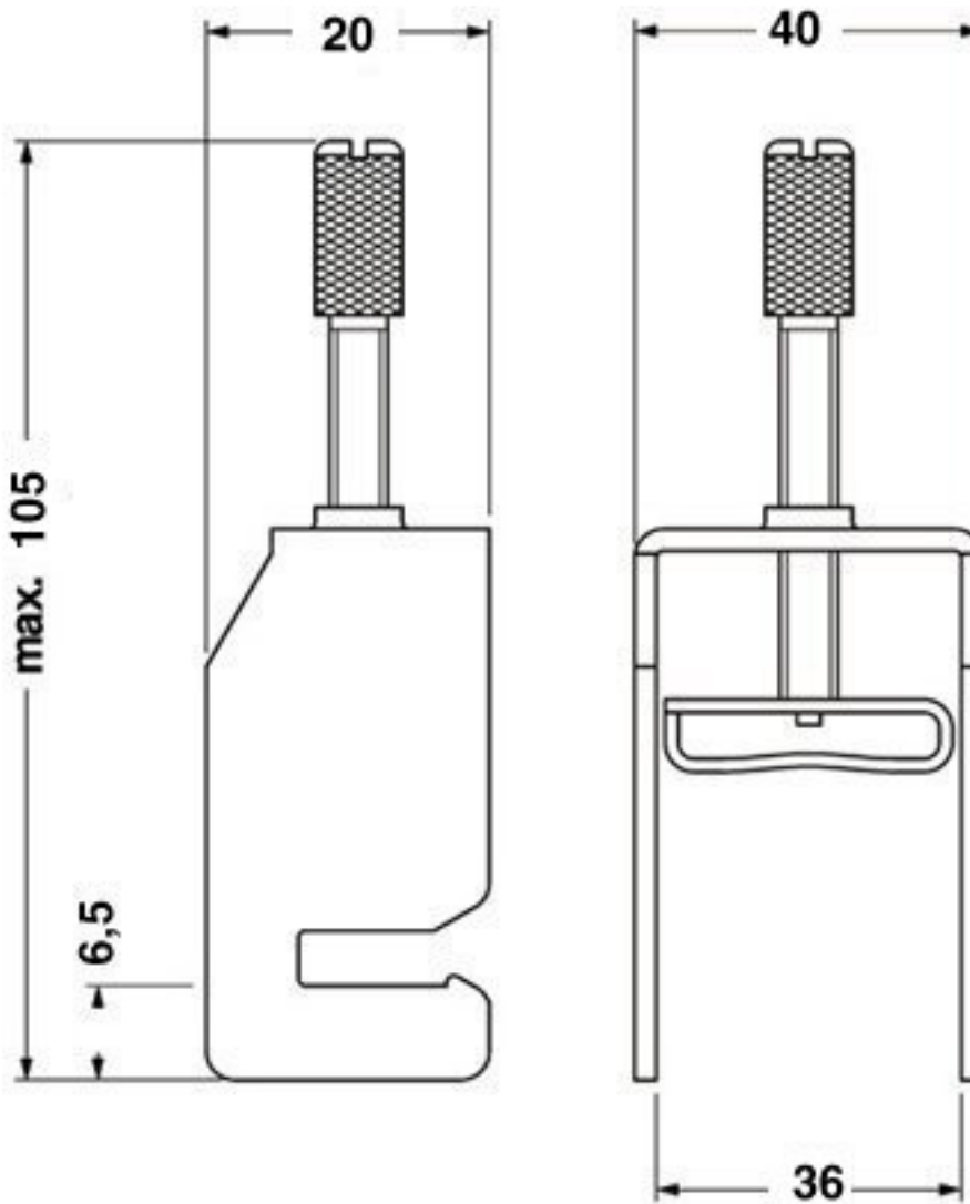
Dimensional drawing
