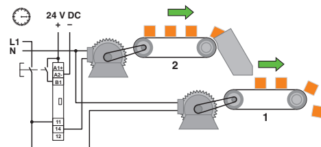
Application drawing
