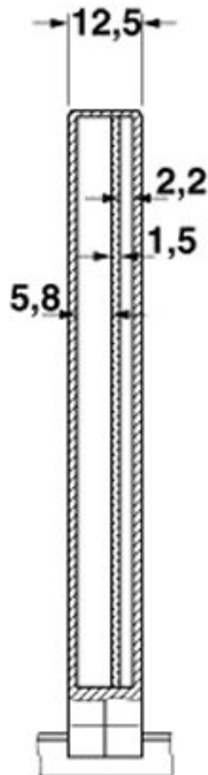
Dimensional drawing
