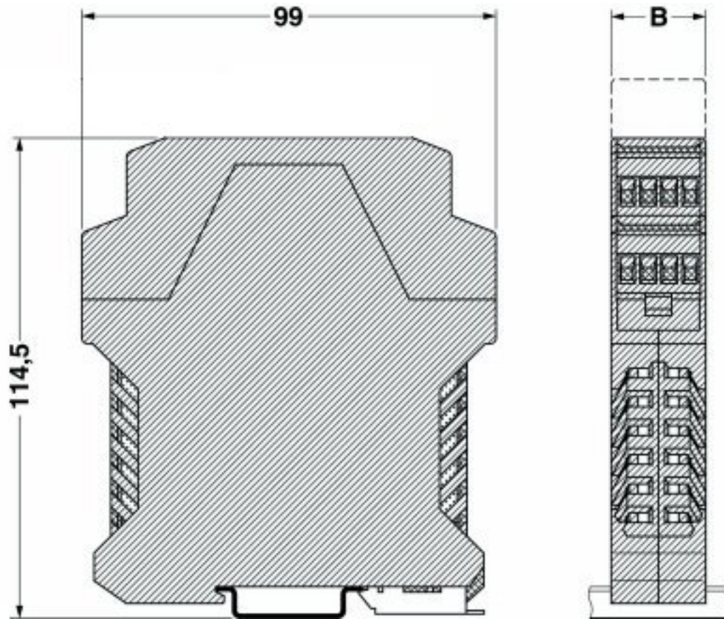
Dimensional drawing
