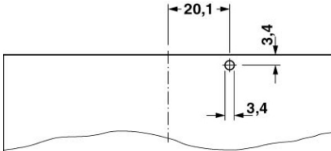
Drilling diagram
