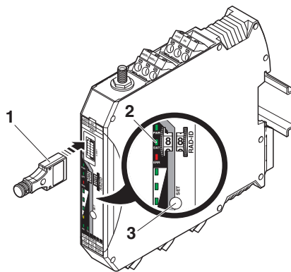
Schematic diagram
