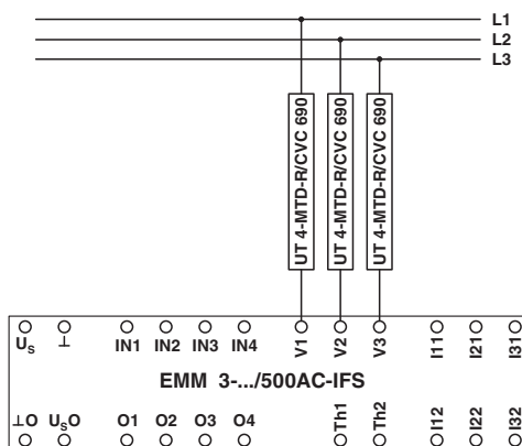
Connection diagram
