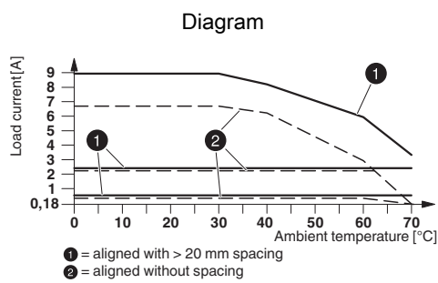
Derating diagram
