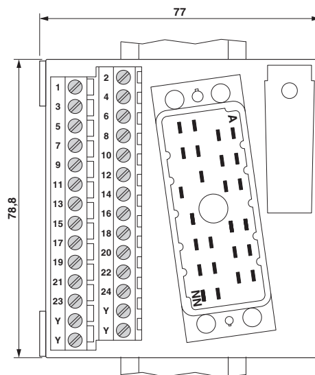
Dimensional drawing
