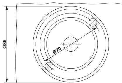
Drilling diagram
