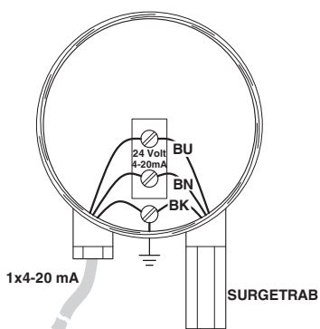
Application drawing
