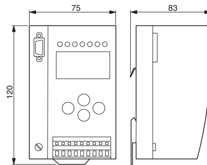
Dimensional drawing
