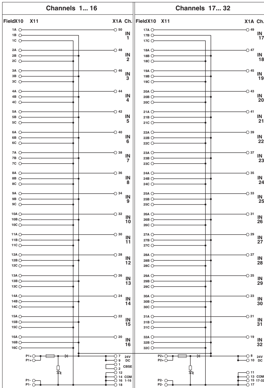
Circuit diagram
