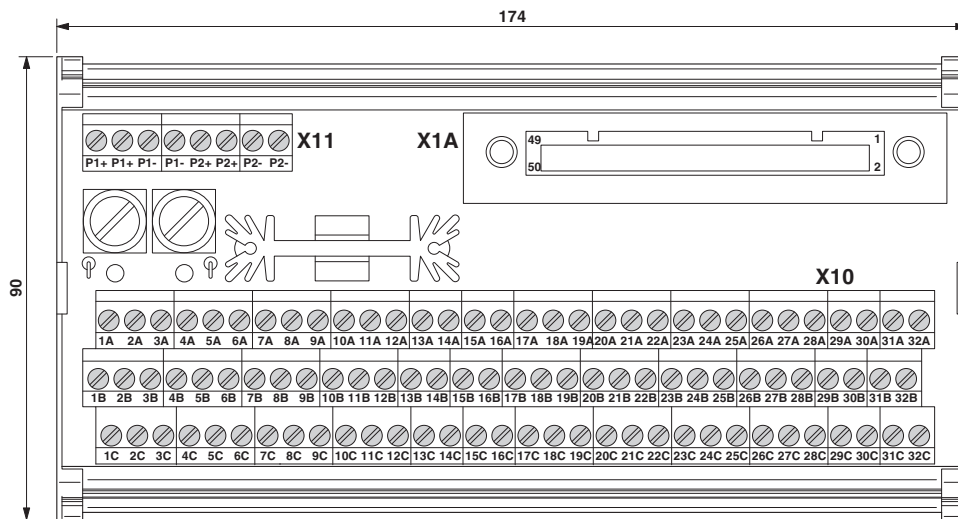
Dimensional drawing
