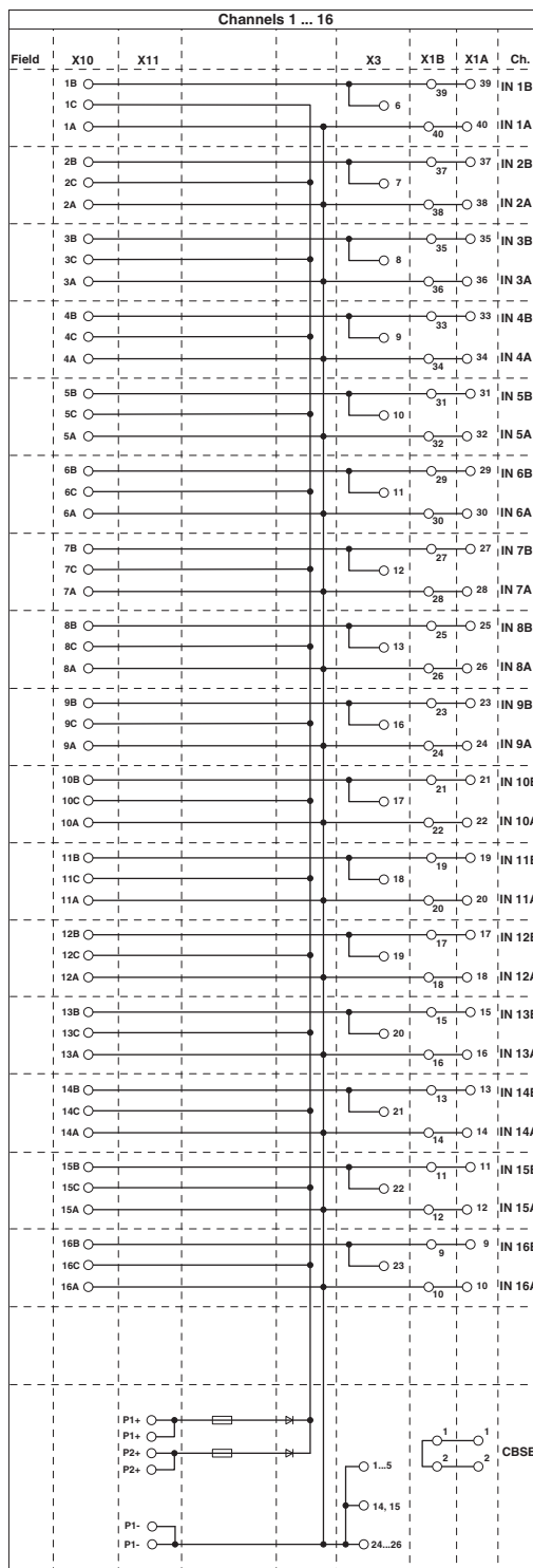
Circuit diagram
