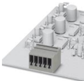
ST-COMBI receptacle, plug-in direction horizontal to the PCB, pitch: 5.2 mm, no. of positions: 6
