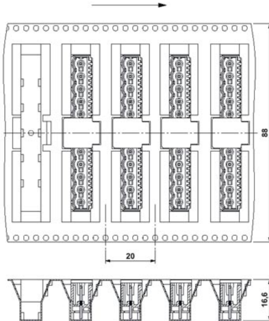
Dimensional drawing
