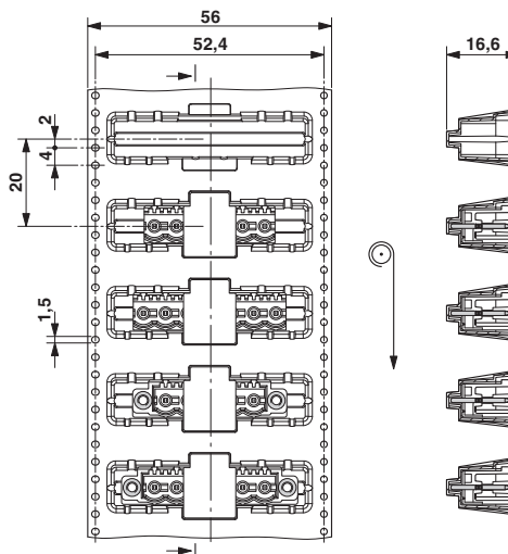
Dimensional drawing
