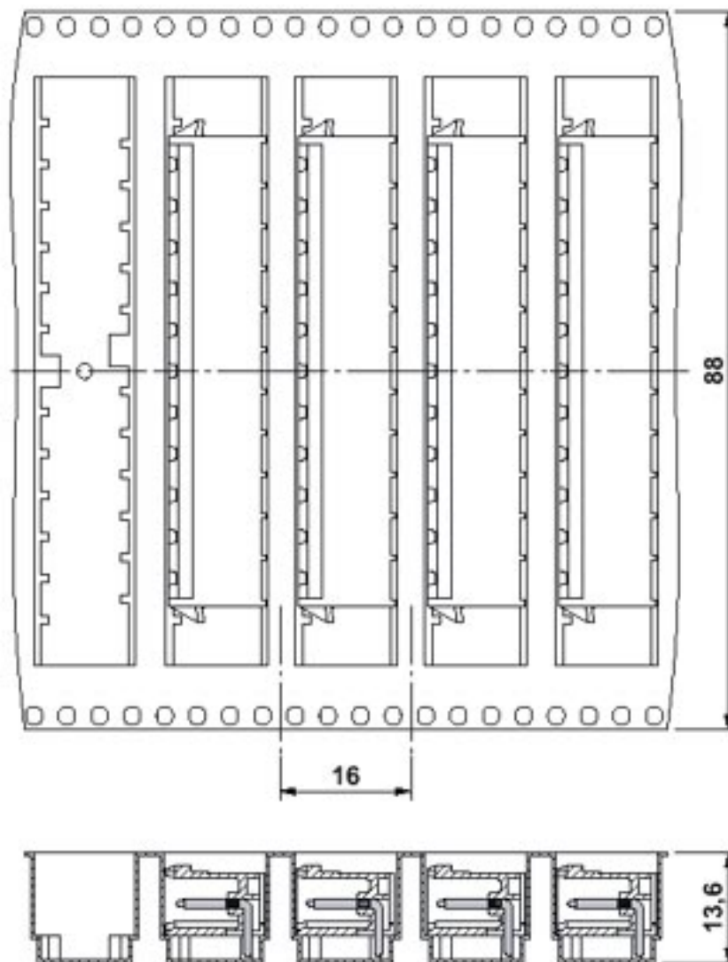
Dimensional drawing
