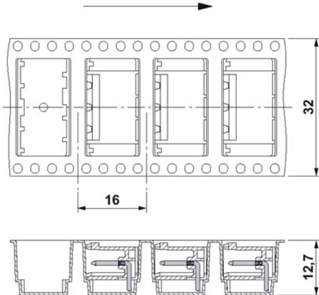
Dimensional drawing
