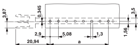
Drilling diagram
