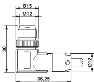
M12 SPEEDCON plug, angled
