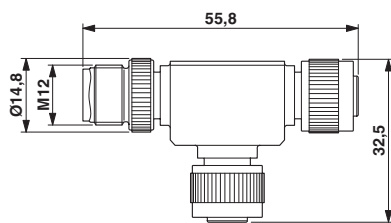
Dimensional drawing
