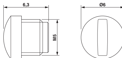
Dimensional drawing
