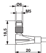
Dimensional drawing
