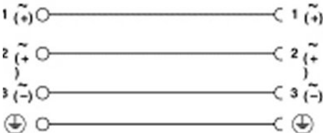
Circuit diagram
