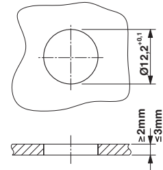
Dimensional drawing
