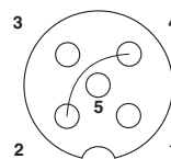
Connector pin assignment M12 socket, 3-pos., bridged, with PE, A-coded, female side view
