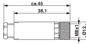
Dimensional drawing
