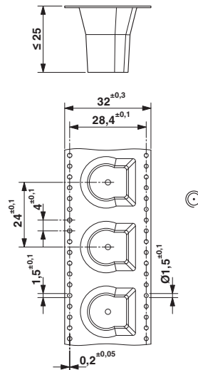
Dimensional drawing
