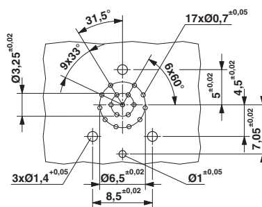
Drilling diagram
