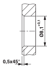
Dimensional drawing
