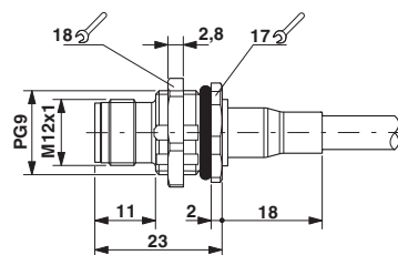
Dimensional drawing
