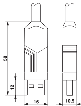
Dimensional drawing
