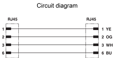
Connector pin assignment plug RJ45
