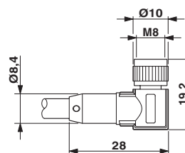
Dimensional drawing
