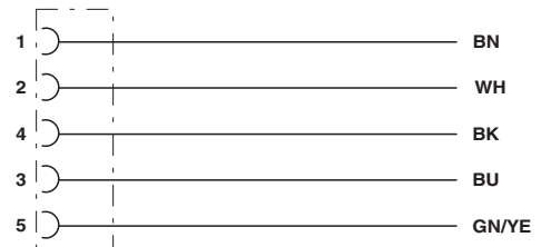
Contact assignment of the M12 sockets
