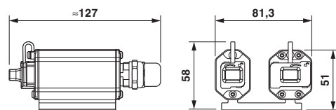
Dimensional drawing
