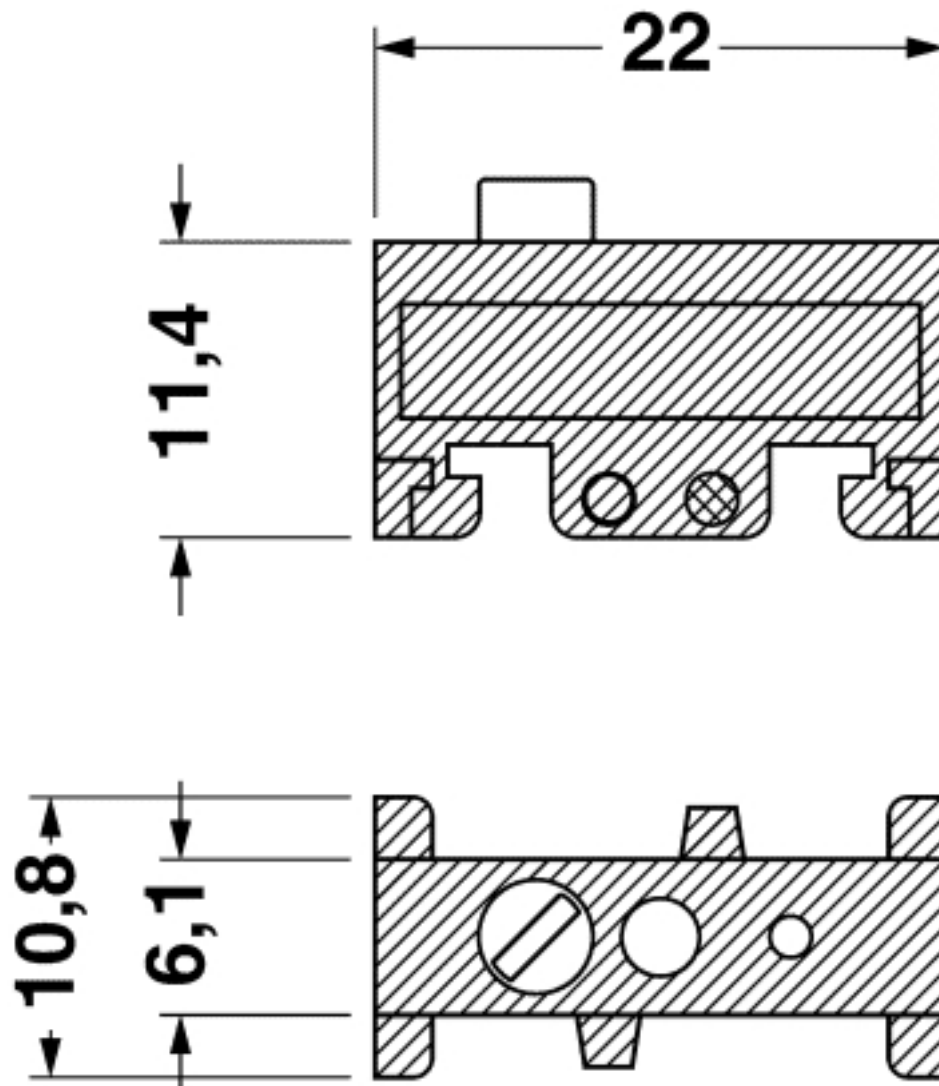
Dimensional drawing
